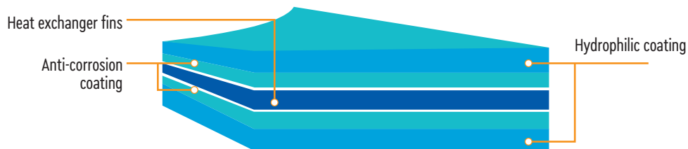
Structure of the double-coated heat exchanger fins
