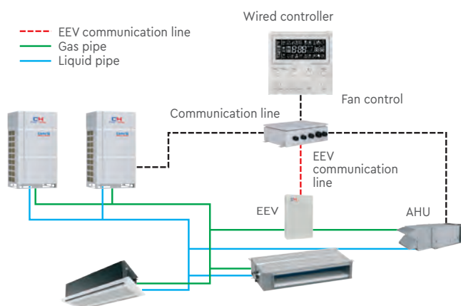
Mixed connection, one AHU kit 2.8 kW ≤ Q x ≤ 28 kW
