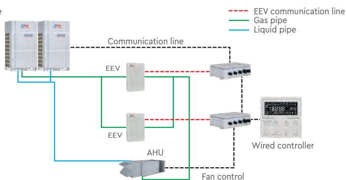
One-to-one connection, few AHU kits for maximal power 84 kW < Q x ≤ 252 kW
