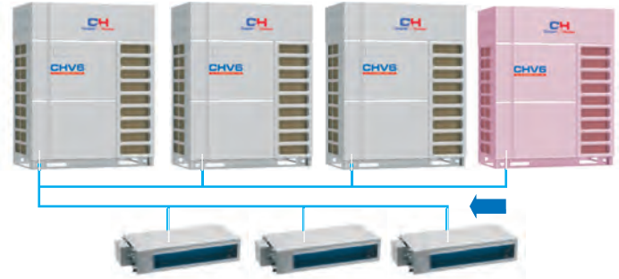
Evacuation of refrigerant in indoor units
